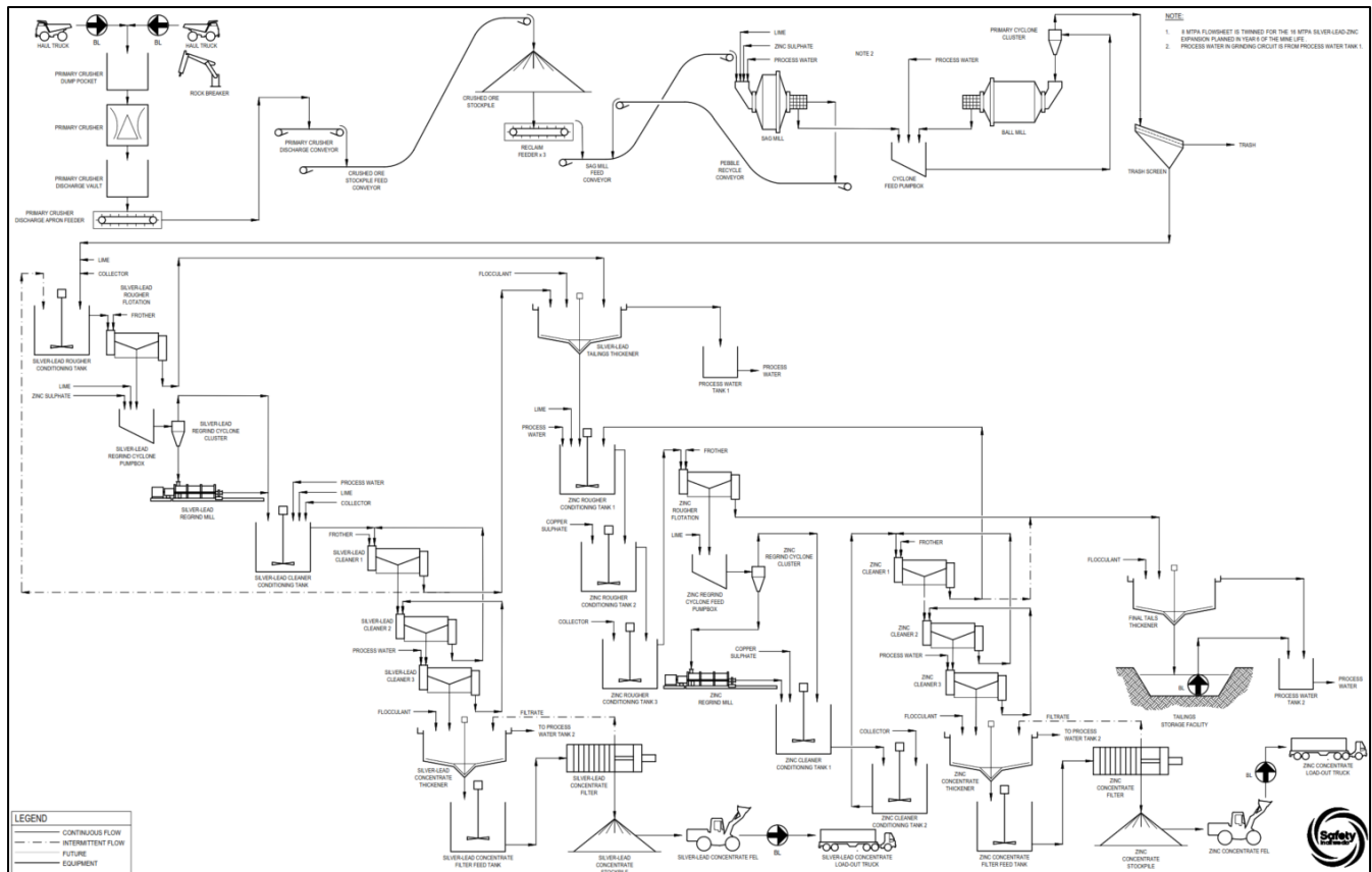
Figure 1-2: Concentrate Process Plant Flowsheet
